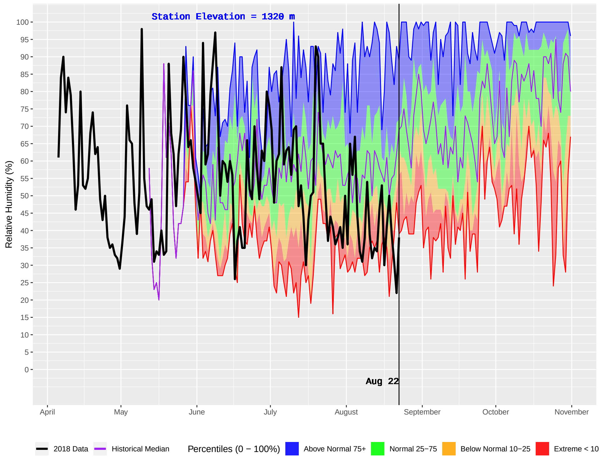
PINE CREEK (938) : Historical (2006–2016) and Current (2018) Daily Relative Humidity
