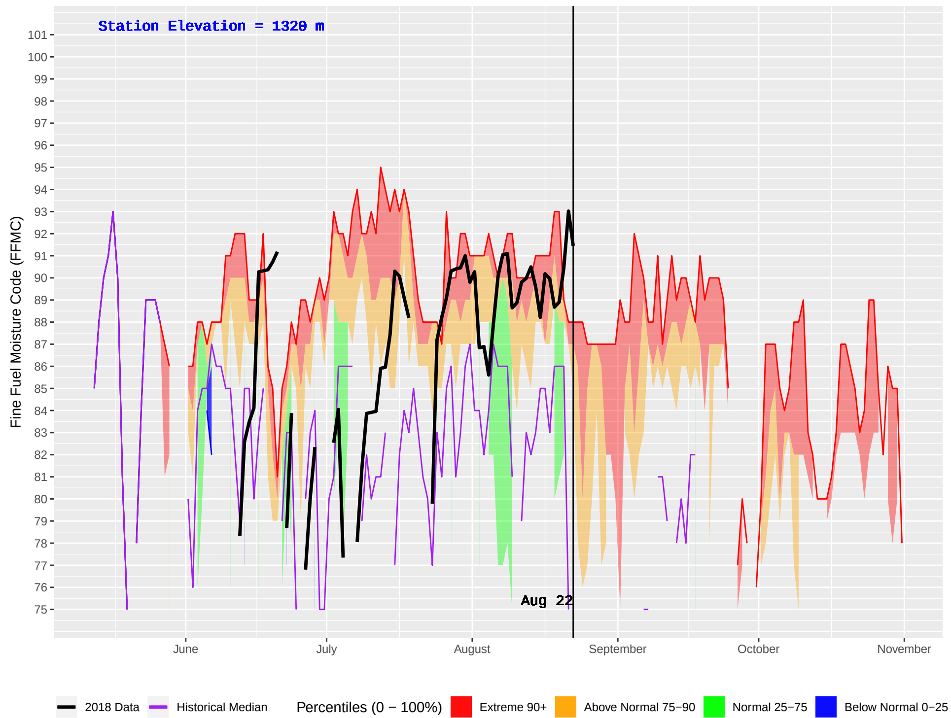
PINE CREEK (938) : Historical (2006–2016) and Current (2018) Daily Fine Fuel Moisture Code (FFMC)
