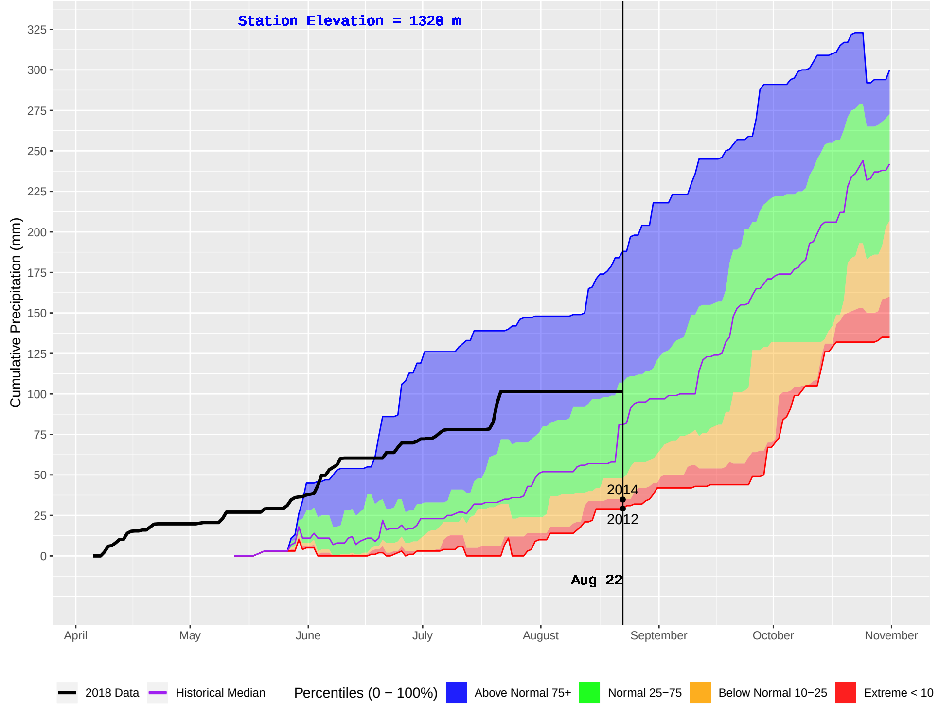
PINE CREEK (938) : Historical (2006–2016) and Current (2018) Daily Cumulative Precipitation
