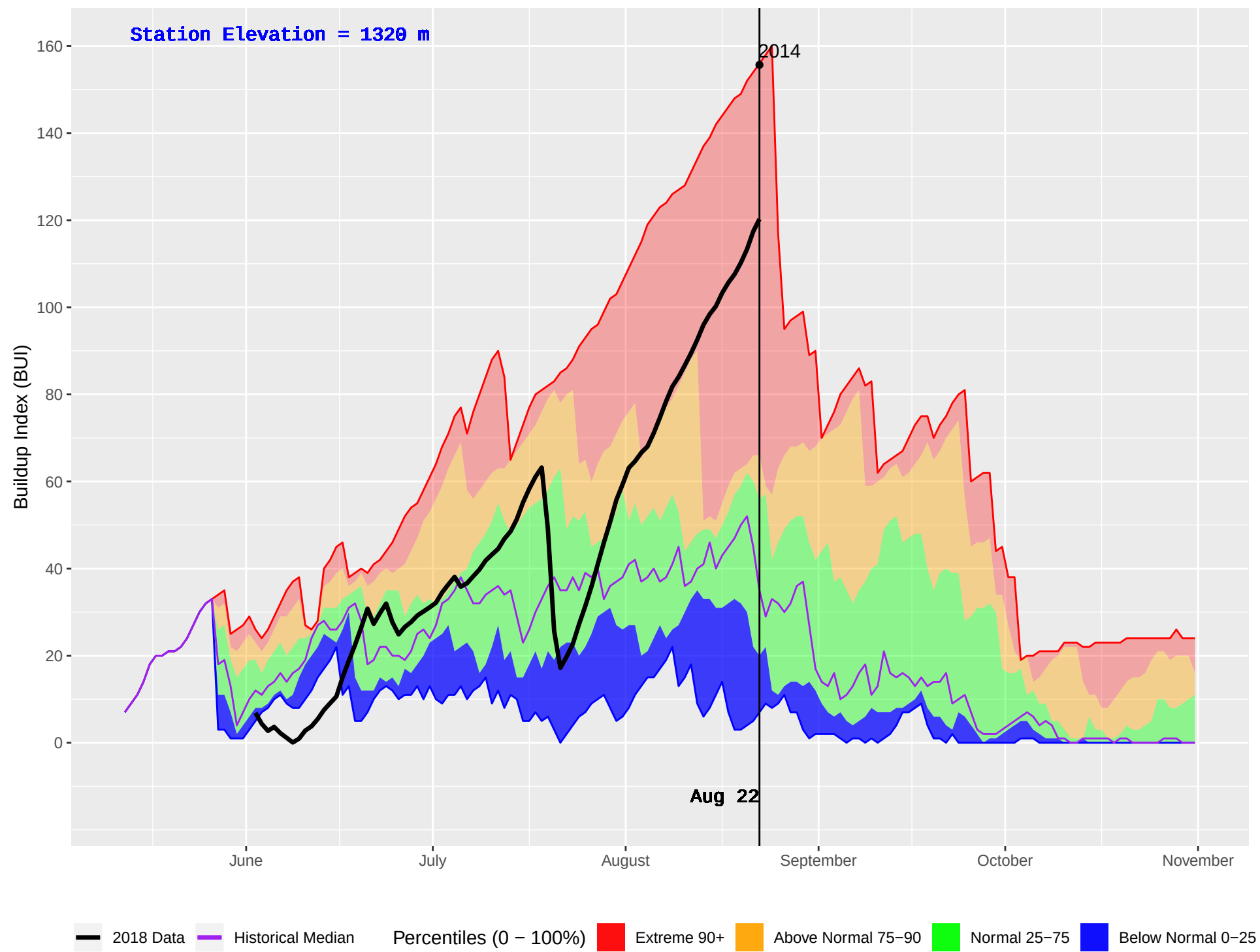
PINE CREEK (938) : Historical (2006–2016) and Current (2018) Daily Buildup Index (BUI)
