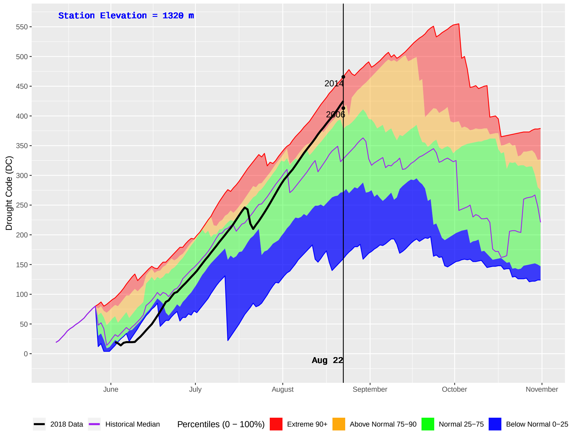
PINE CREEK (938) : Historical (2006–2016) and Current (2018) Daily Drought Code (DC)
