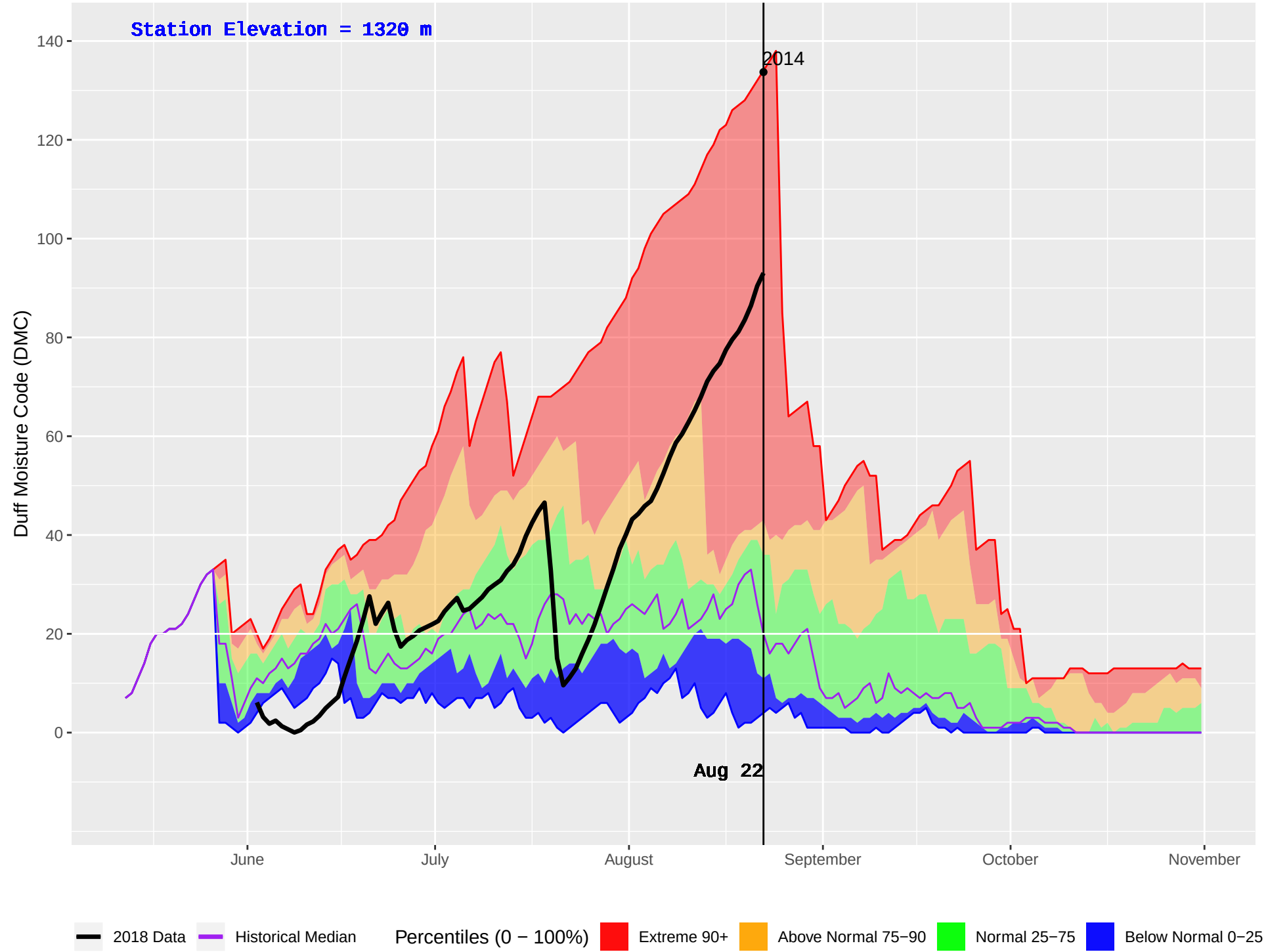
PINE CREEK (938) : Historical (2006–2016) and Current (2018) Daily Duff Moisture Code (DMC)
